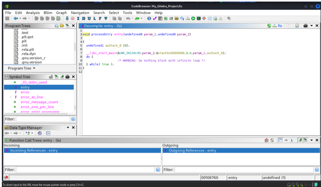
Figure 4: Decompiled C-like pseudocode of the entry function
